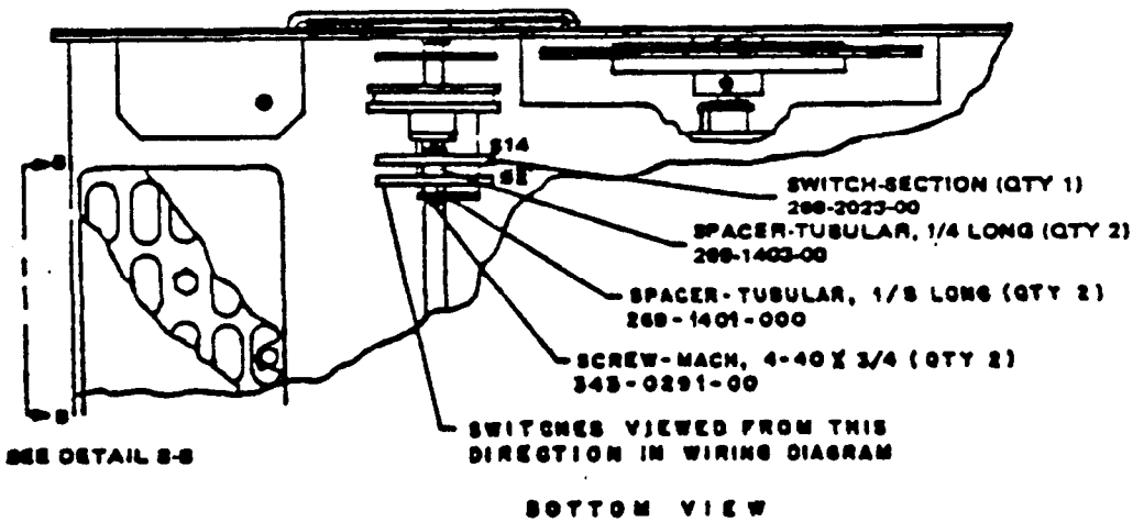
KWM-2 Amateur Transceiver, Additional Crystal Board, Installation Drawing Figure 1 (Sheet 1 of 3)
