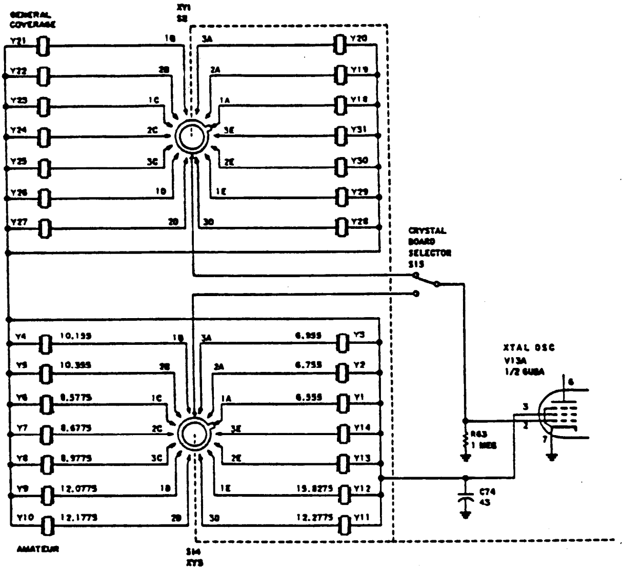
KWM-2 Amateur Transceiver Additional Crystal Board, Schematic Diagram Figure 2
